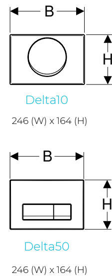
Delta Flush Plates
