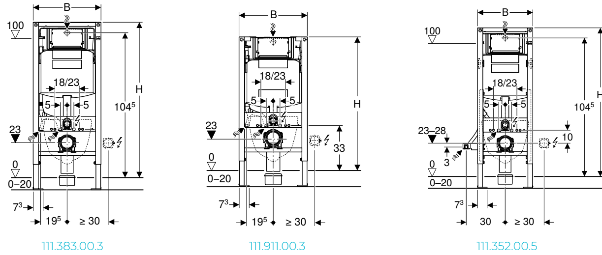
Duofix Frame with Sigma concealed cistern
