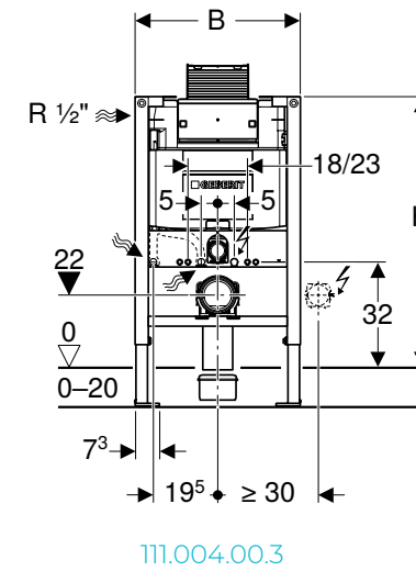
Duofix Frame with Omega concealed cistern
