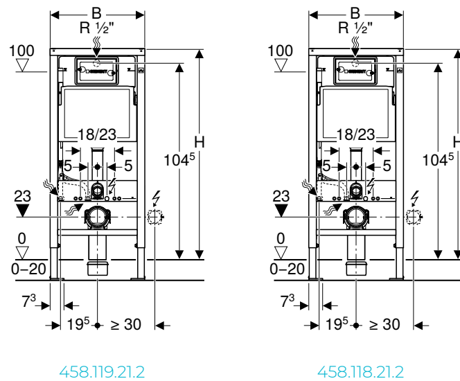
Duofix Frame with Delta concealed cistern
