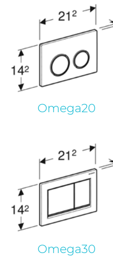
Omega Flush Plates
