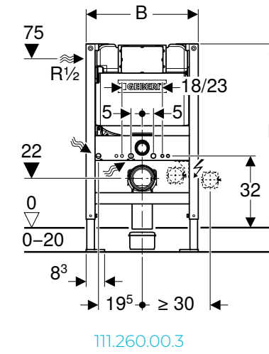
Duofix Frame with Kappa concealed cistern
